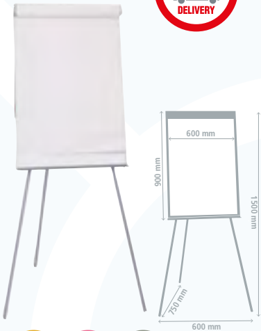
Non-Magnetic Telescopic Flip Chart Easel 3500 600(w) x 1500mm(h)
