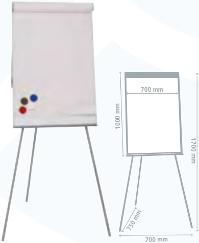
Magnetic Telescopic Flip Chart Easel 95010 700(w) x 1700mm(h)
